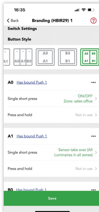
Figure 22.6 Switch configuration-2
