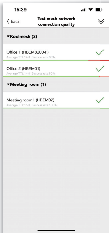
Figure 12.1 Mesh quality
