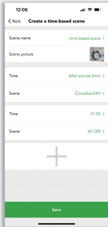
Figure 6.39 Time-based scene
