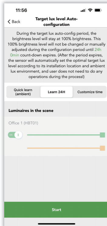
Figure 6.20.3 Closed loop
