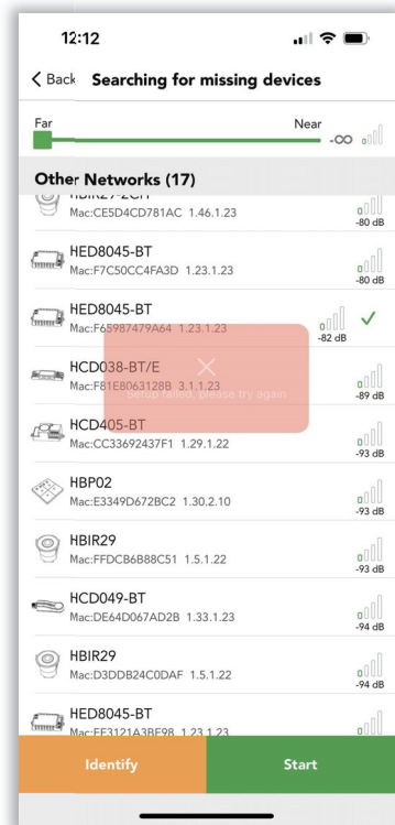
Figure 7.5 Setup failed
