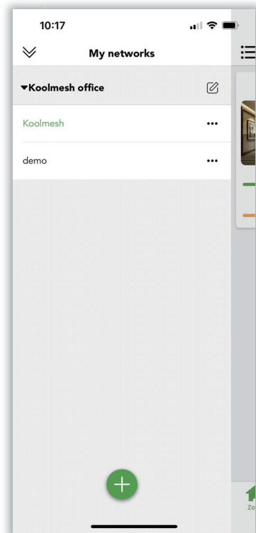
Figure 3.12 Modification done
