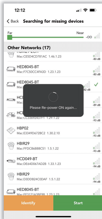
Figure 7.4 Devices-3
