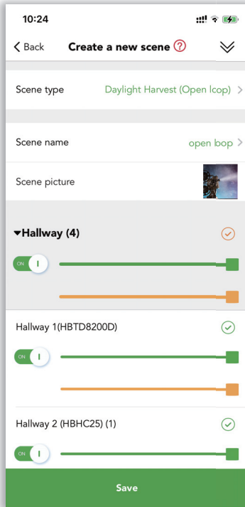
Figure 6.10 Create scene
