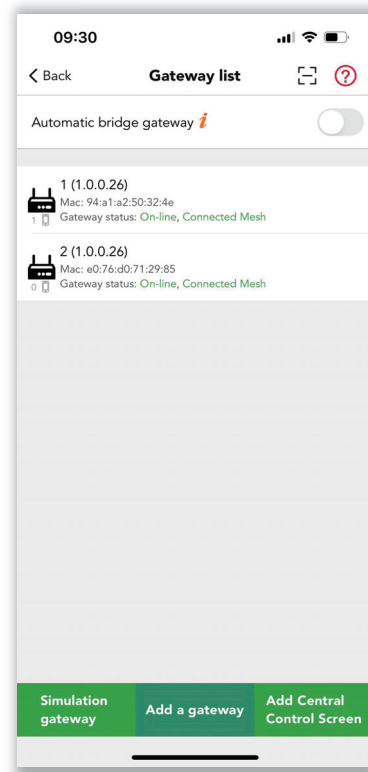
Figure 13.3 Gateway list
