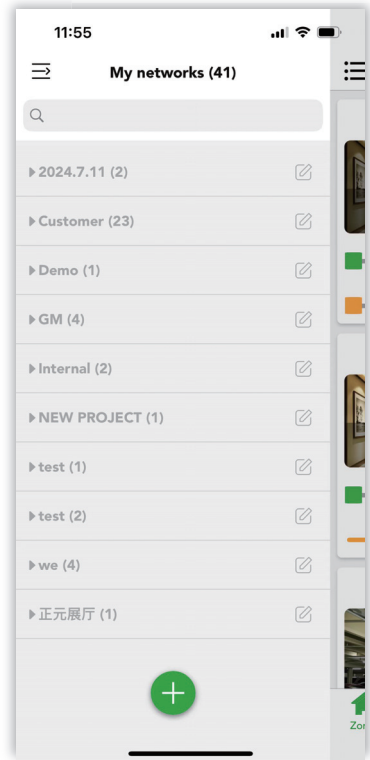
Figure 3.7.4 Hide project
