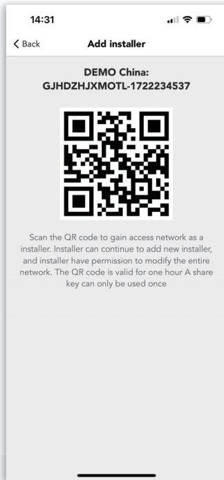
Figure 11.2.1 Add installerr
