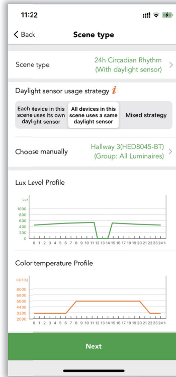
Figure 6.32 Settings
