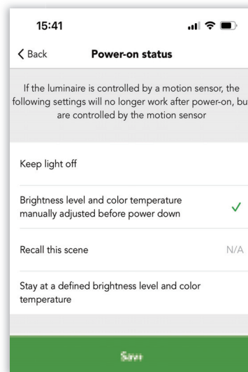
Figure 8.4 Power-on status
