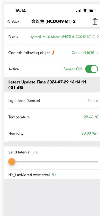
Figure 20.6 Add Multi-Meter-2
