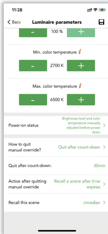
Figure 6.49 Luminaire settings
