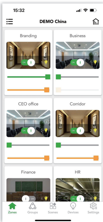
Figure 3.5 Home page
