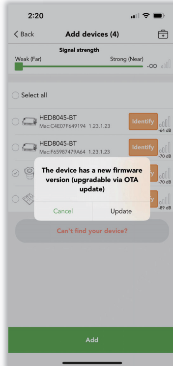
Figure 4.3 Add device-1
