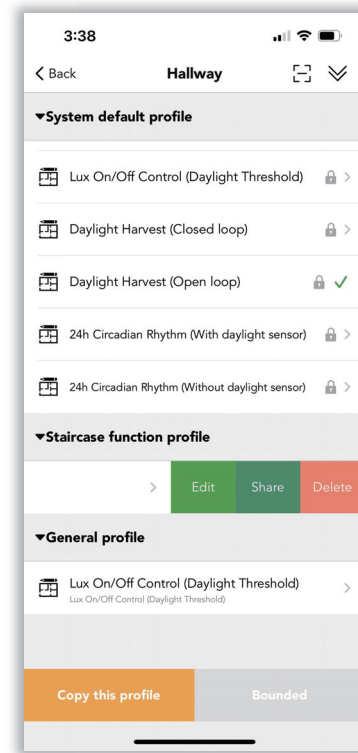
Figure 17.3 Change profile
