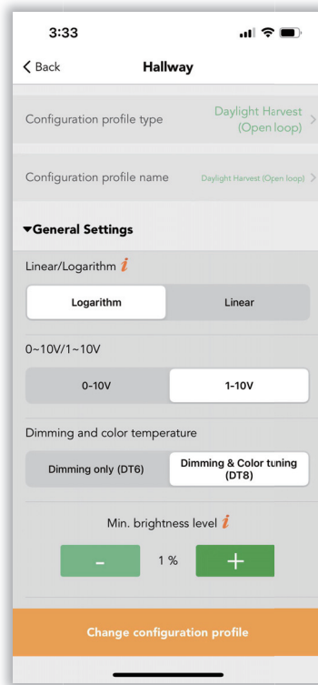
Figure 17.2 Modify profile
