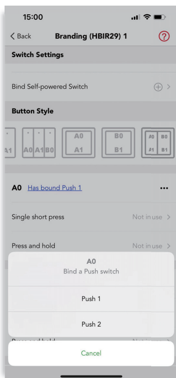
Figure 22.5 Switch configuration-1
