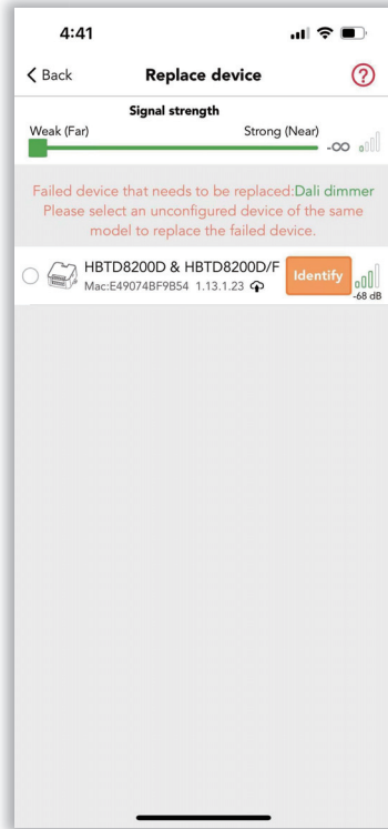
Figure 7.8 Replace device
