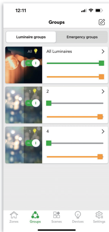
Figure 5.1 Groups
