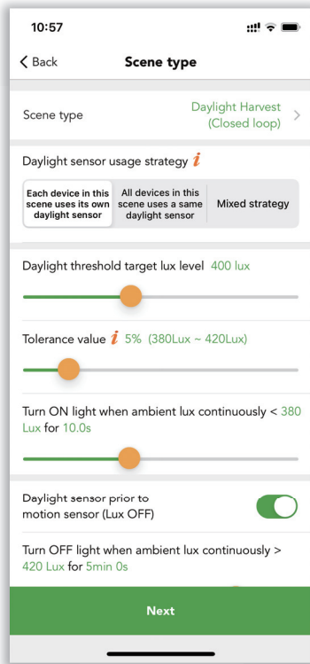
Figure 6.20 Closed loop
