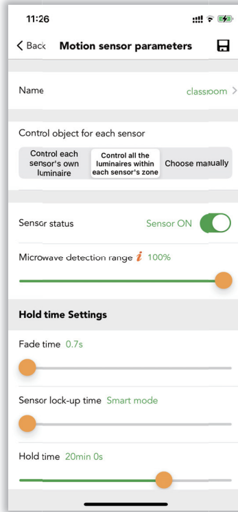
Figure 6.43 Sensor settings
