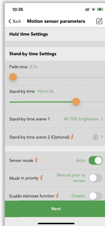
Figure 6.18 Scene saved
