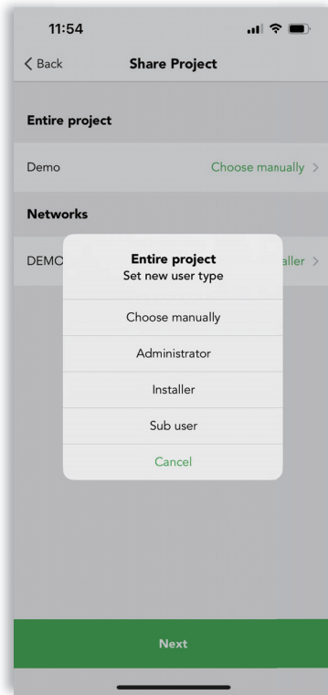
Figure 3.7.3 Share project
