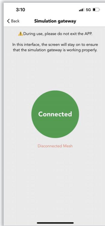
Figure 13.12 Simulation gateway-2
