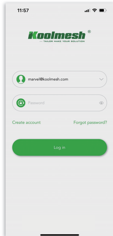
Figure 1.3 Log in
