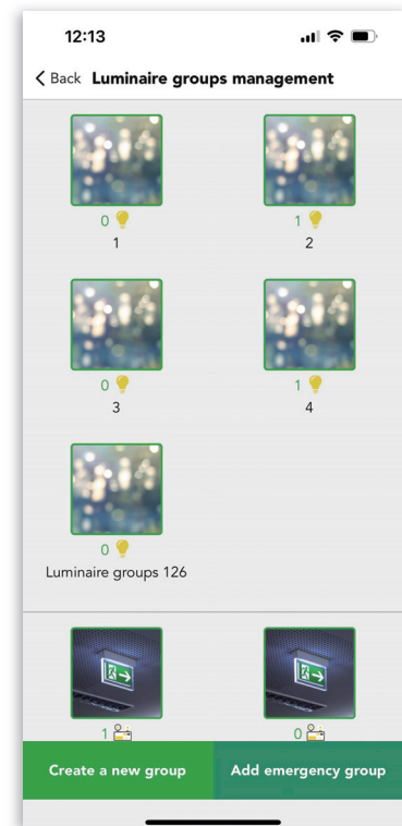
Figure 5.2 Groups management
