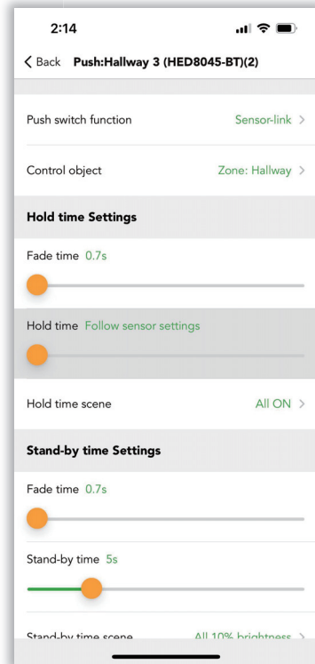
Figure 21.3 Push settings
