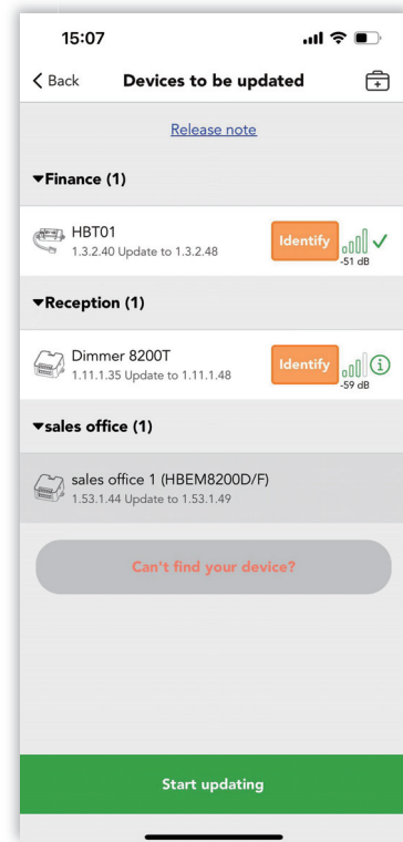
Figure 12.4 Release
