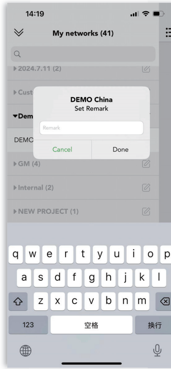
Figure 3.8.2 Set Remark
