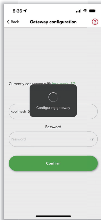
Figure 13.2 Gateway configuration
