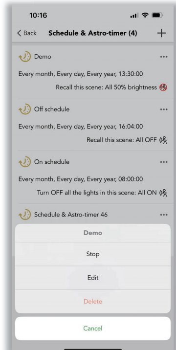
Figure 14.3 Edit schedule
