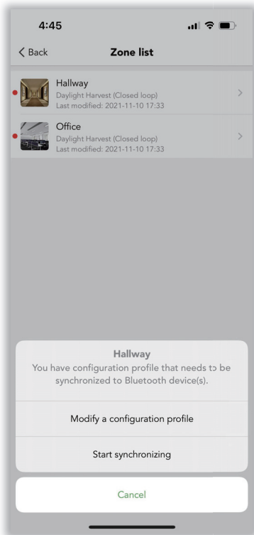
Figure 17.1 Zone list
