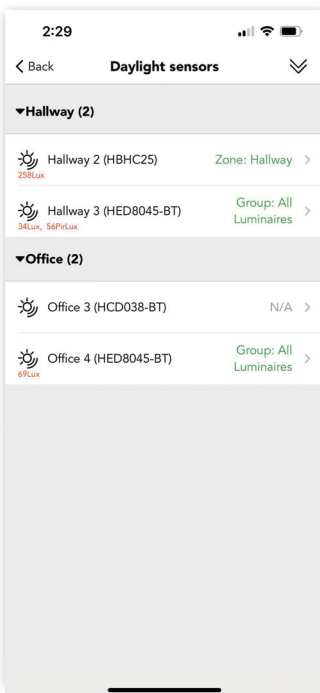
Figure 20.1 Daylight sensors
