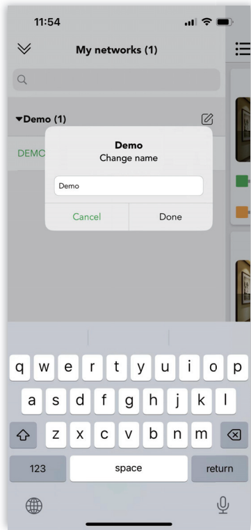
Figure 3.7.2 Change name
