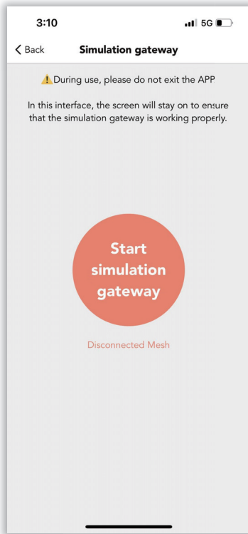
Figure 13.11 Simulation gateway-1
