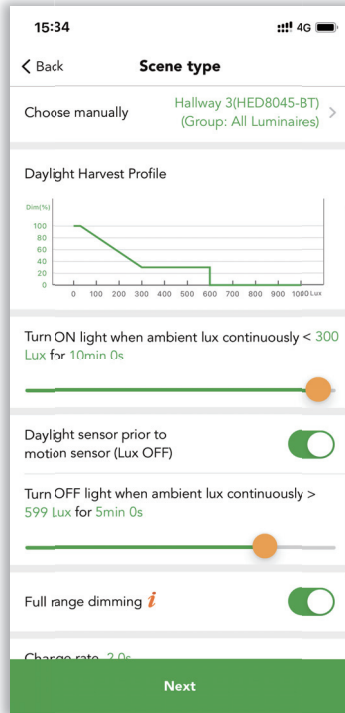
Figure 6.11 Scene setting
