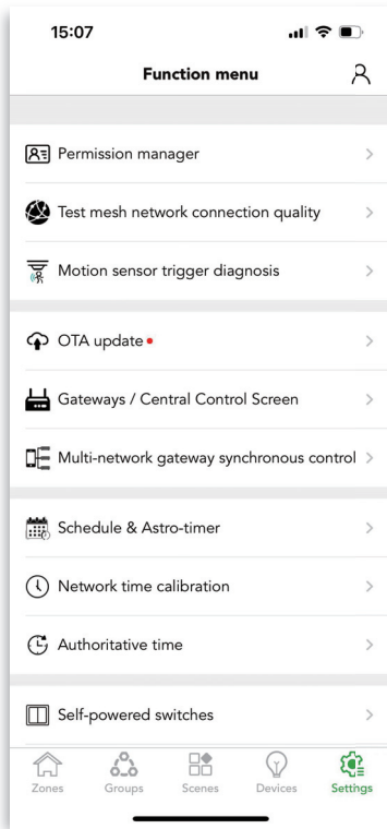
Figure 12.2 OTA-1
