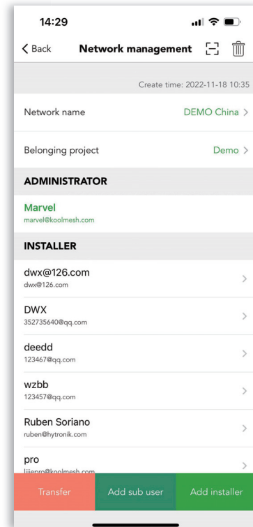
Figure 3.9.1 Network mangement
