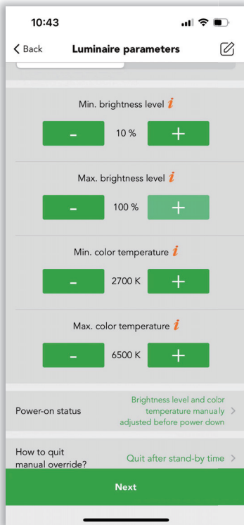
Figure 6.23 Save
