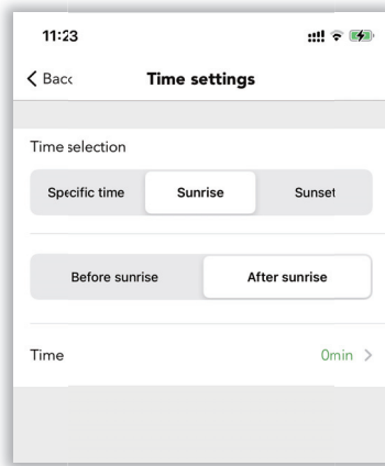
Figure 6.37 First scene
