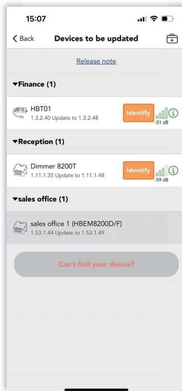
Figure 12.3 OTA-2
