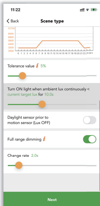
Figure 6.33 Lux disabled
