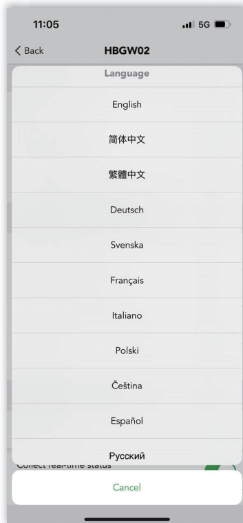
Figure 13.13 Language
