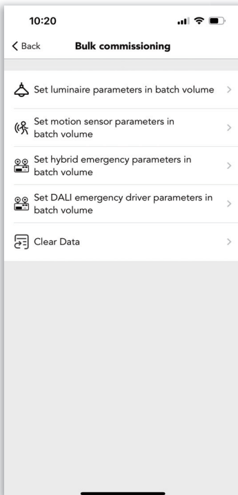
Figure 6.13 Bulk commissioning
