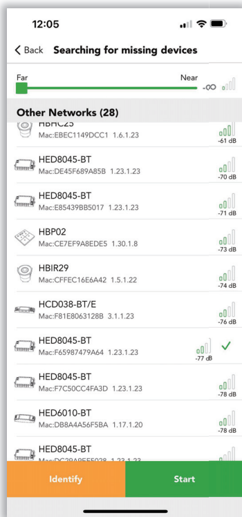
Figure 7.3 Devices-2
