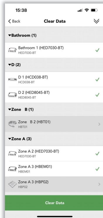
Figure 18.7 Device list
