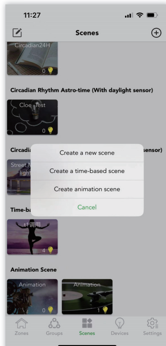
Figure 6.2 Create scenes
