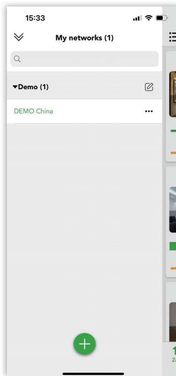
Figure 3.6 My networks
