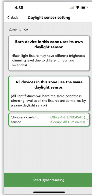
Figure 17.11 Start synchronizing
