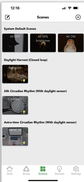
Figure 6.20.1 Closed loop
