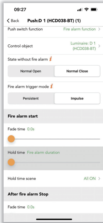
Figure 21.4.2 Firm alarm
