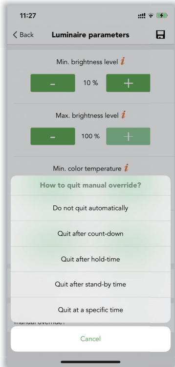
Figure 6.48 Quit options
