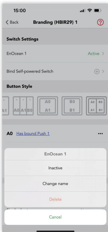
Figure 22.4 Function
