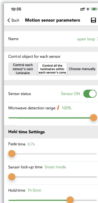
Figure 6.15 Parameters setting
