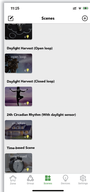
Figure 6.41 Scenes overview
