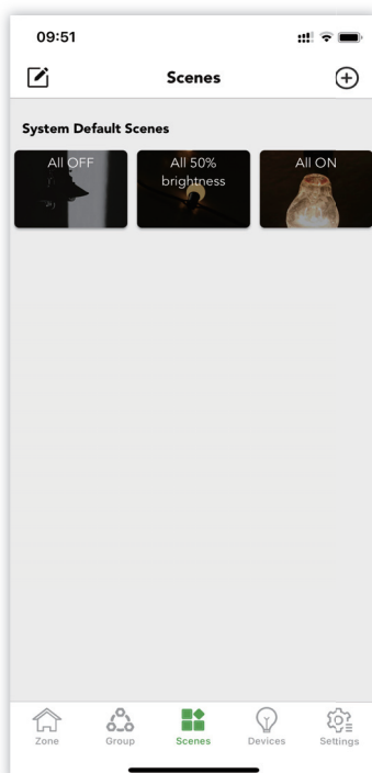
Figure 6.1 Scenes
