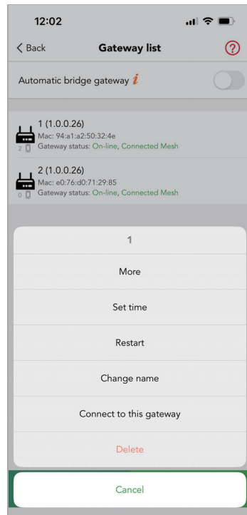
Figure 13.5.1 Function
